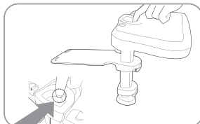
Pushing the button (protrusion) of the Foot Plate hole inside, join the Foot Plate and the Height Control Bar
